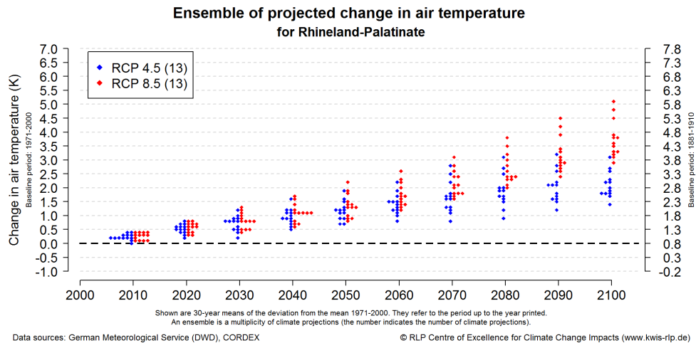
Fig. 1: Ensemble of projected change in air temperature in the calendar year, (Source: German Meteorological Service, CORDEX, © Rhineland-Palatinate Centre of Excellence for Climate Change Impacts)
