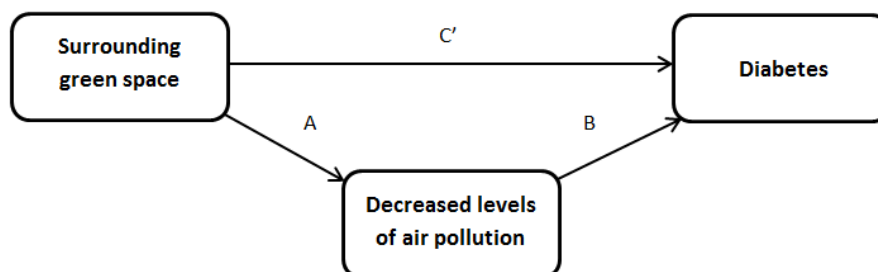
Fig. 1: Schematic overview of the direct ( C' ) and indirect effect ( AB ) of surrounding green space on diabetes. (Source: J. O. Klompaker et al.)
