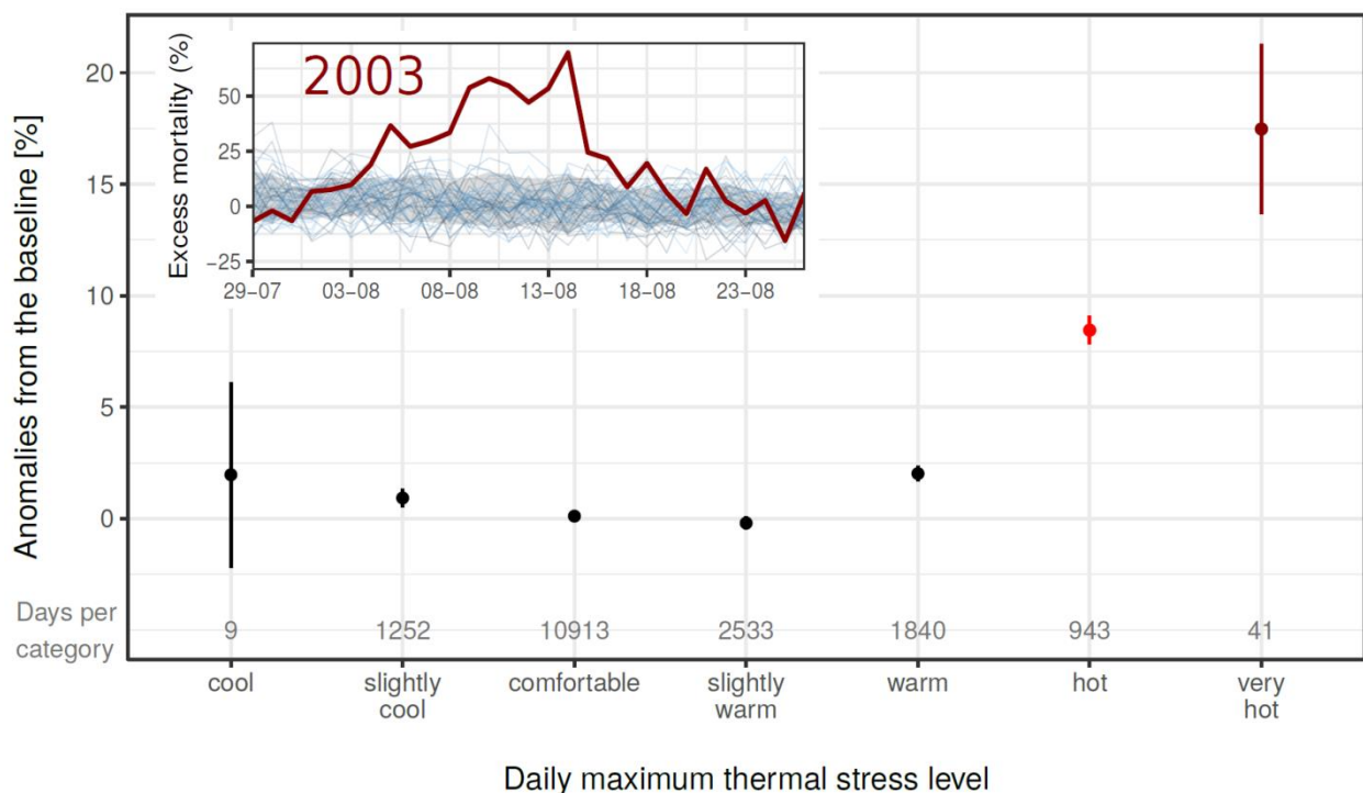
Fig. 1: Relationship between the daily maximum heat stress (Perceived Temperature) and mortality in Baden-Württemberg (South-West Germany) for the period 1968-2015. Subpanel: Mortality time series for Baden-Württemberg during the August 2003 heat wave. Thin lines and shading: Individual years and background variability 1968-2015. (Source: German Meteorological Service)
