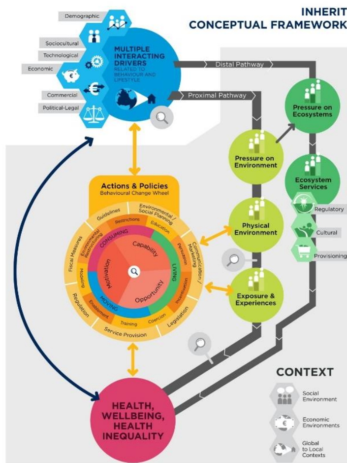
Fig. 1: INHERIT Model (Source: INHERIT Baseline Review)
