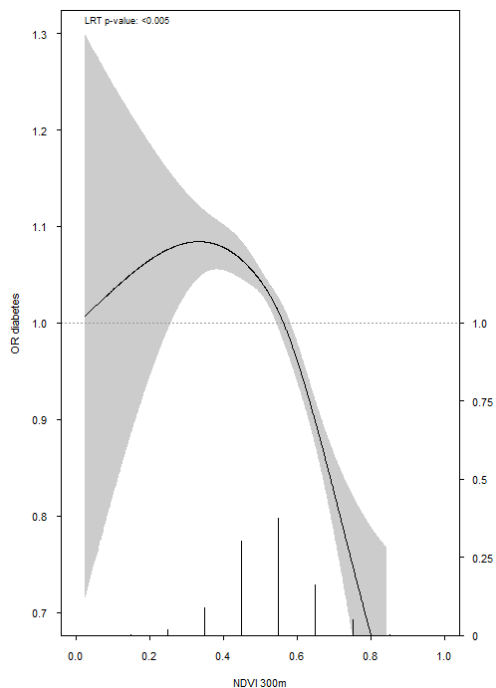
Fig. 2: Estimated exposure-response curves (solid line) and 95% CIs (grey area) for the odds of diabetes for NDVI in a 300m buffer. At the left x-axis the OR is shown, at the right x-axis the probability distribution of the NDVI is shown. (Source: J.O. Klompmaker et al.)
