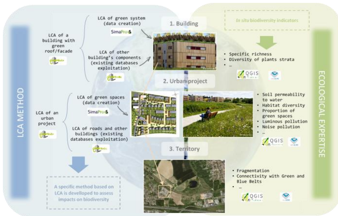
Fig. 1: Hybrid methodology for biodiversity assessment (Source: Aline Brachet)
