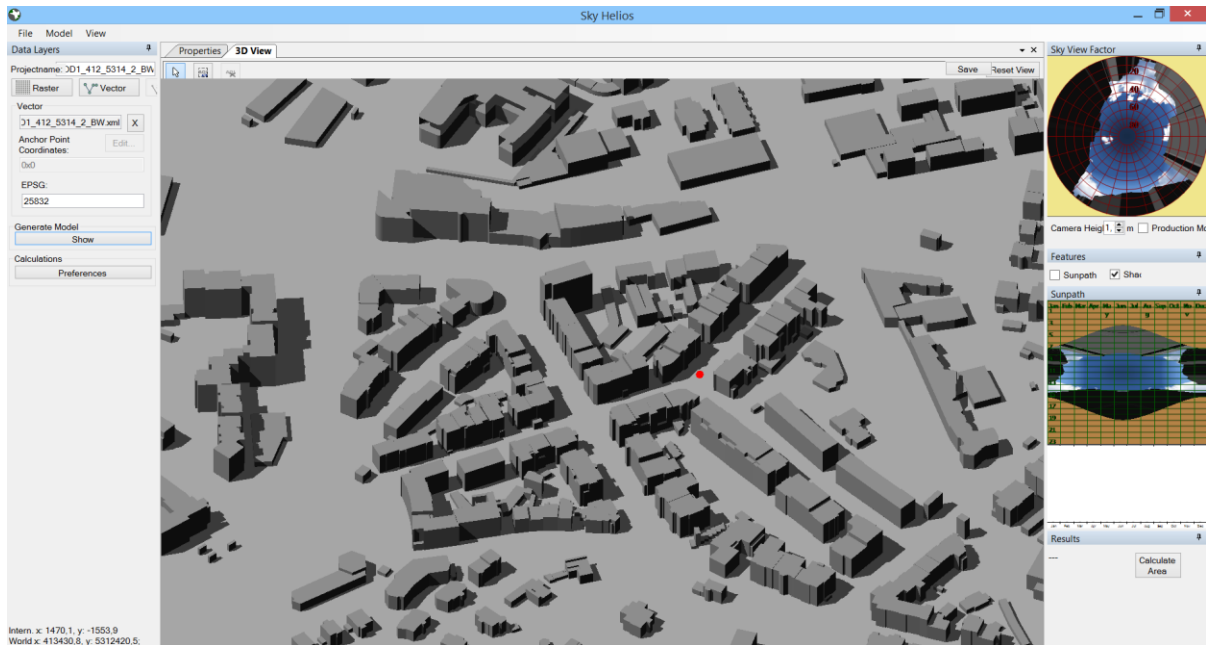
Fig. 1: Shading at 14:34 LST calculated for an excerpt of the City of Freiburg, represented by a CityGML building geometry model using the SkyHelios model. (Source: German Meteorological Service).
